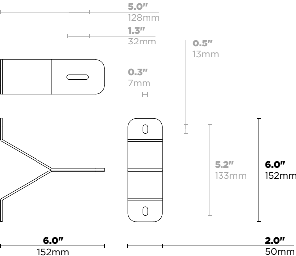
(ADJUSTABILITY AND MOUNTING DIMENSIONS IN GREY)
