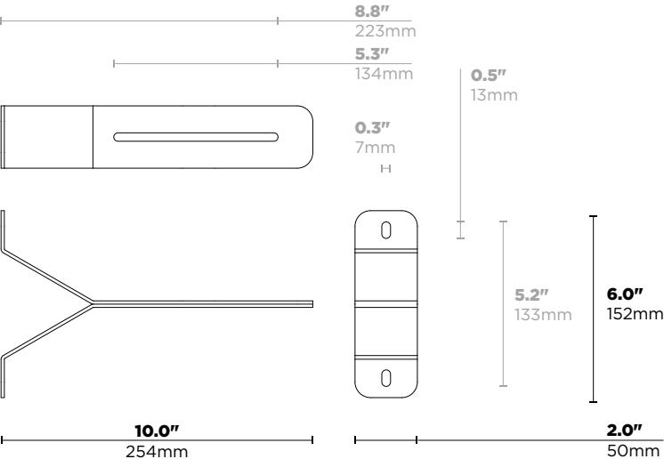
(ADJUSTABILITY AND MOUNTING DIMENSIONS IN GREY)
