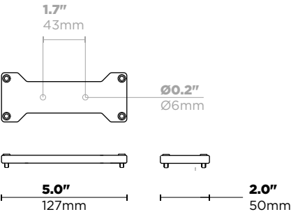
(ADJUSTABILITY AND MOUNTING DIMENSIONS IN GREY)
